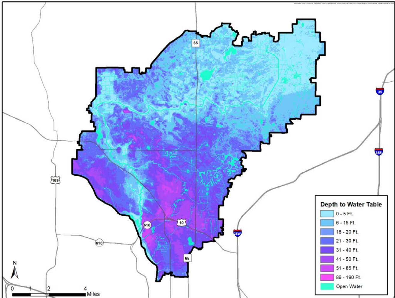
Figure 3.14. District hydrology
