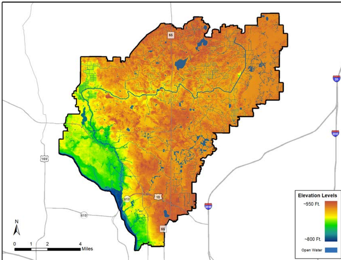
Figure 3.41. CCWD topography
