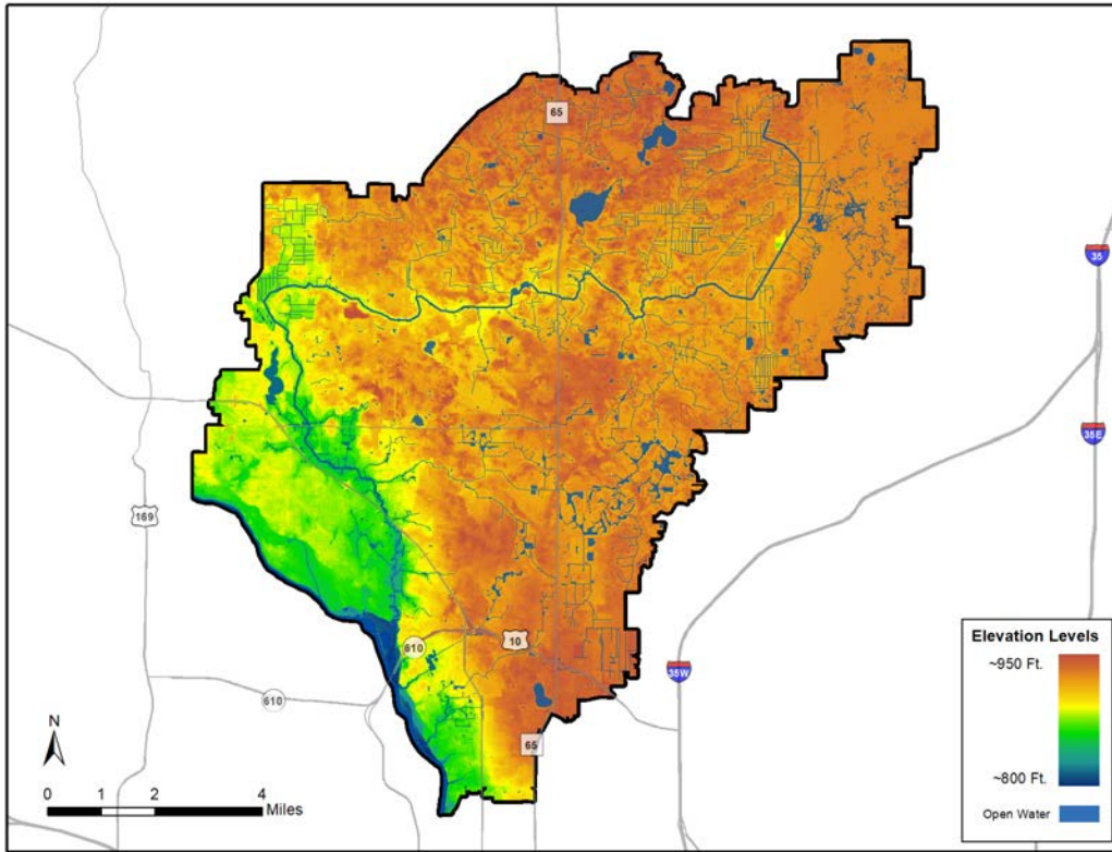
Figure 3.02. CCWD topography
