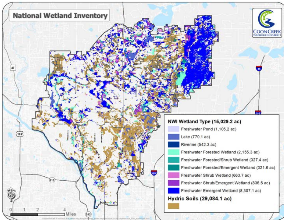
Figure 3.38. NWI wetlands map
