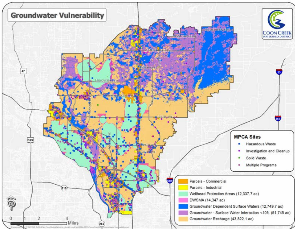
Figure 3.24. Groundwater pollution vulnerability
