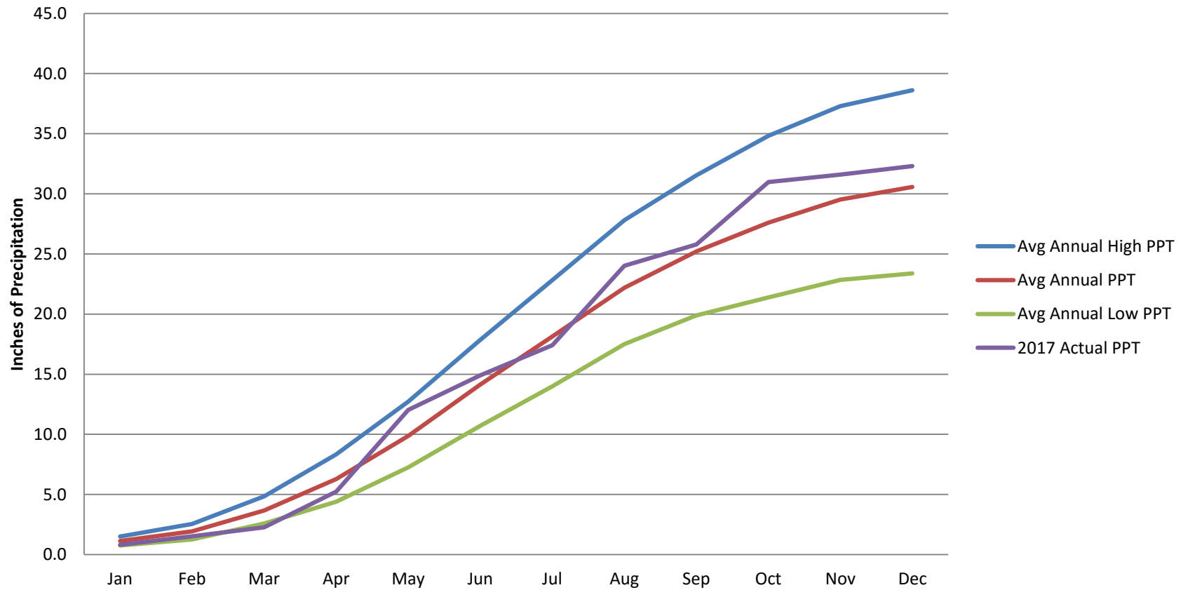
Year-To-Date Precipitation
