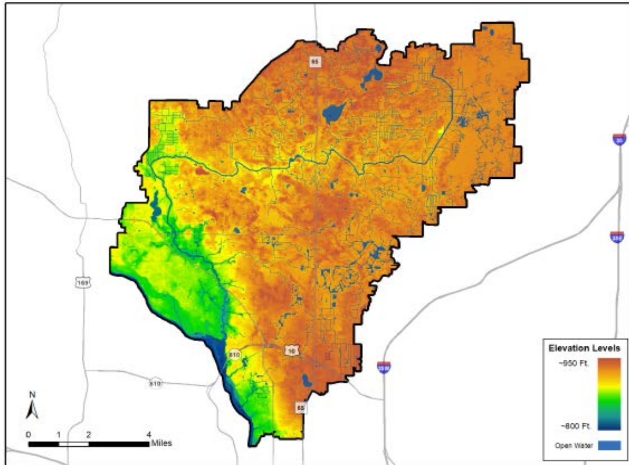
Figure 3.13. CCWD topography
