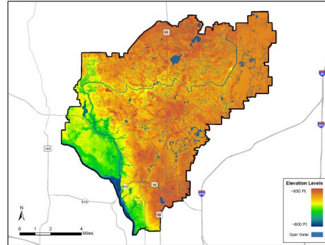
Figure 3.02. CCWD topography
